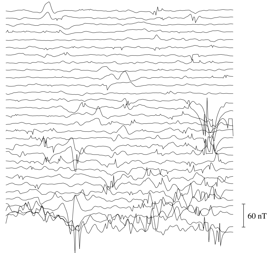
b) Traceplot of despiked Caesium magnetometer data.
